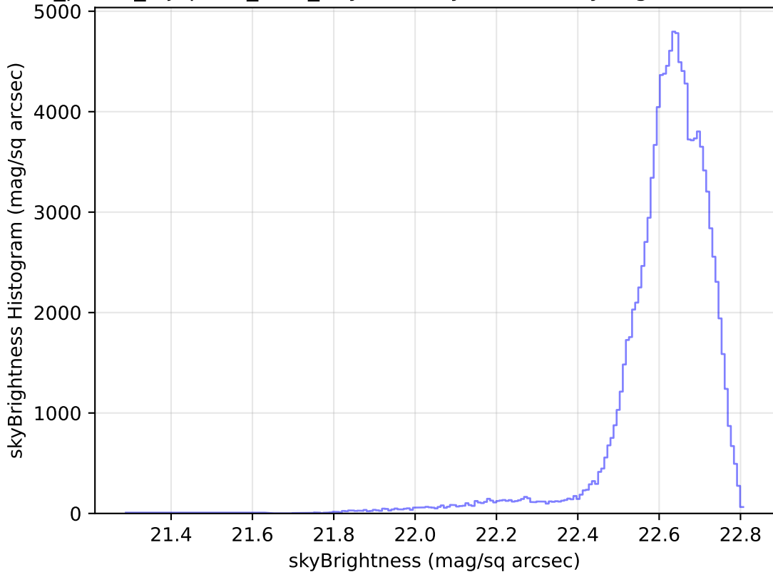
roll_pause_mjdp270_v3.4_10yrs All sky u band: skyBrightness Histogram
