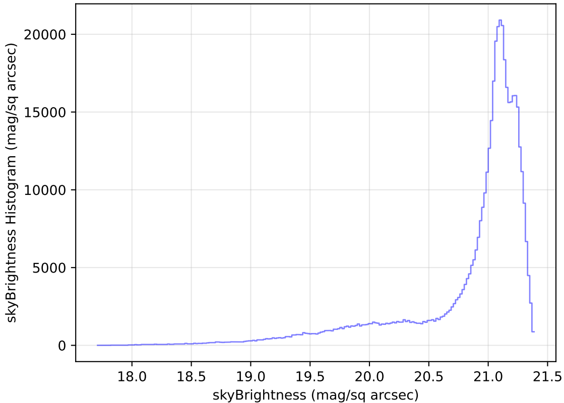
roll_pause_mjdp270_v3.4_10yrs All sky r band: skyBrightness Histogram
