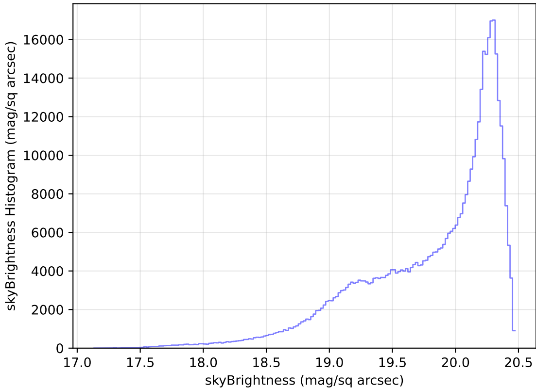
roll_pause_mjdp270_v3.4_10yrs All sky i band: skyBrightness Histogram
