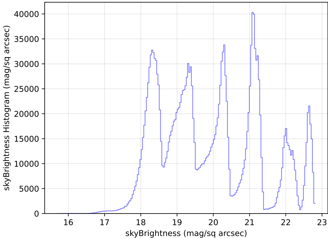
roll_pause_mjdp270_v3.4_10yrs All sky all bands: skyBrightness Histogram
