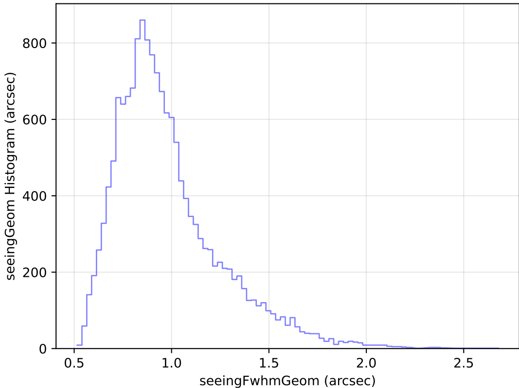
roll_pause_mjdp270_v3.4_10yrs Yr 1 u band: seeingGeom Histogram
