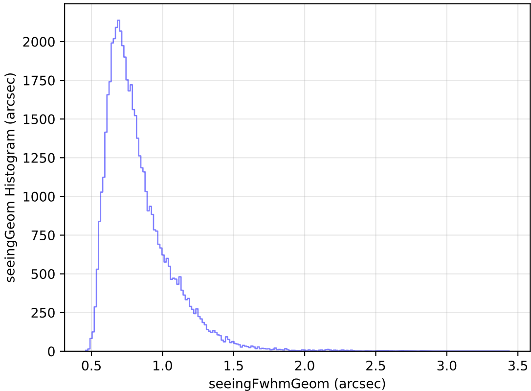
roll_pause_mjdp270_v3.4_10yrs Yr 1 i band: seeingGeom Histogram
