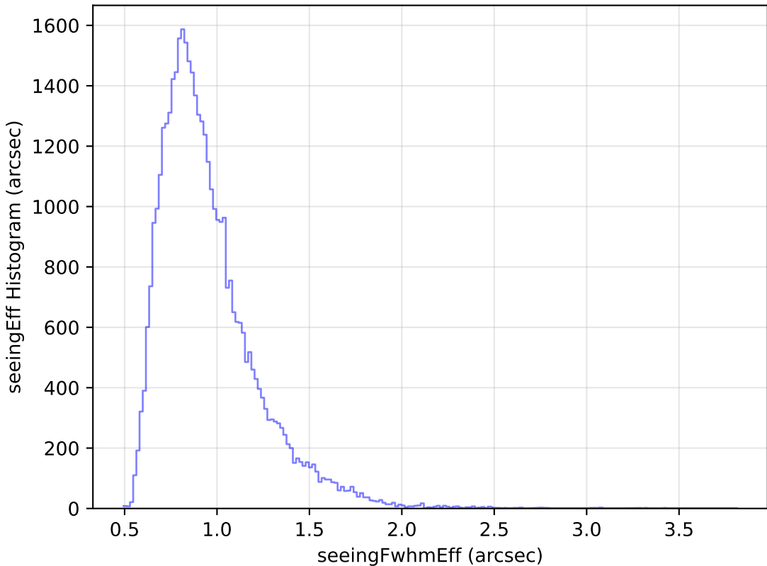
roll_pause_mjdp270_v3.4_10yrs Yr 1 z band: seeingEff Histogram
