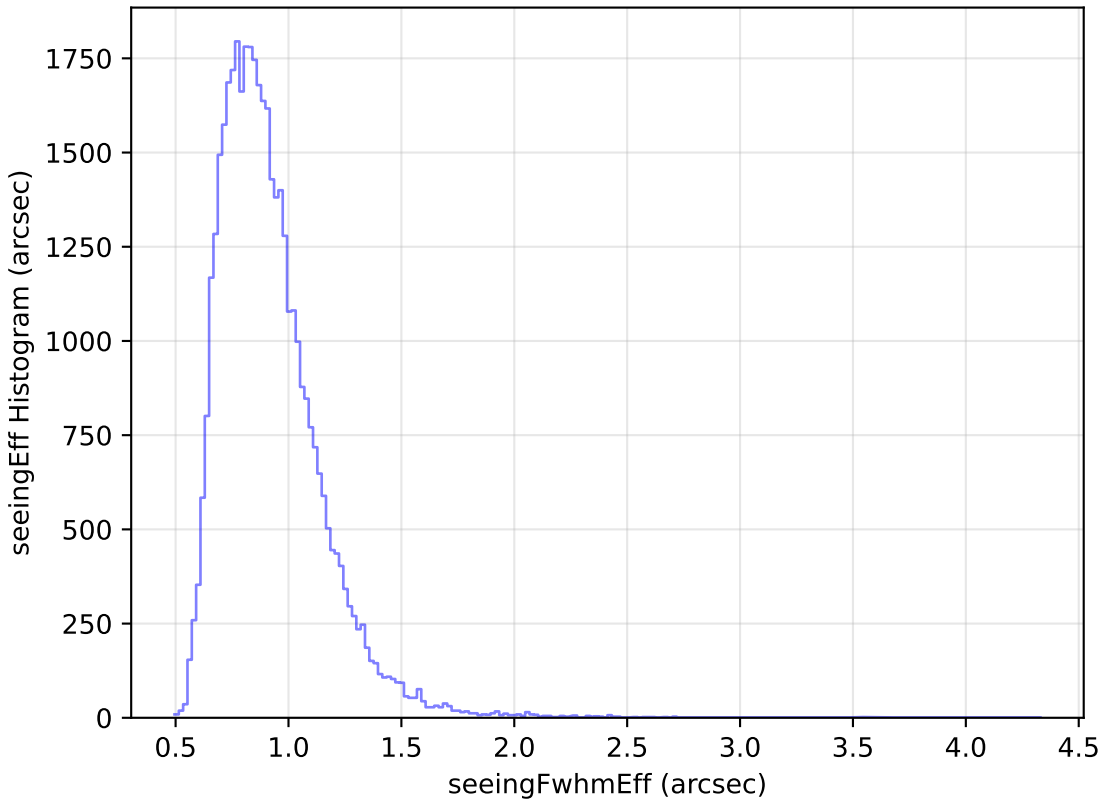
roll_pause_mjdp270_v3.4_10yrs Yr 1 y band: seeingEff Histogram
