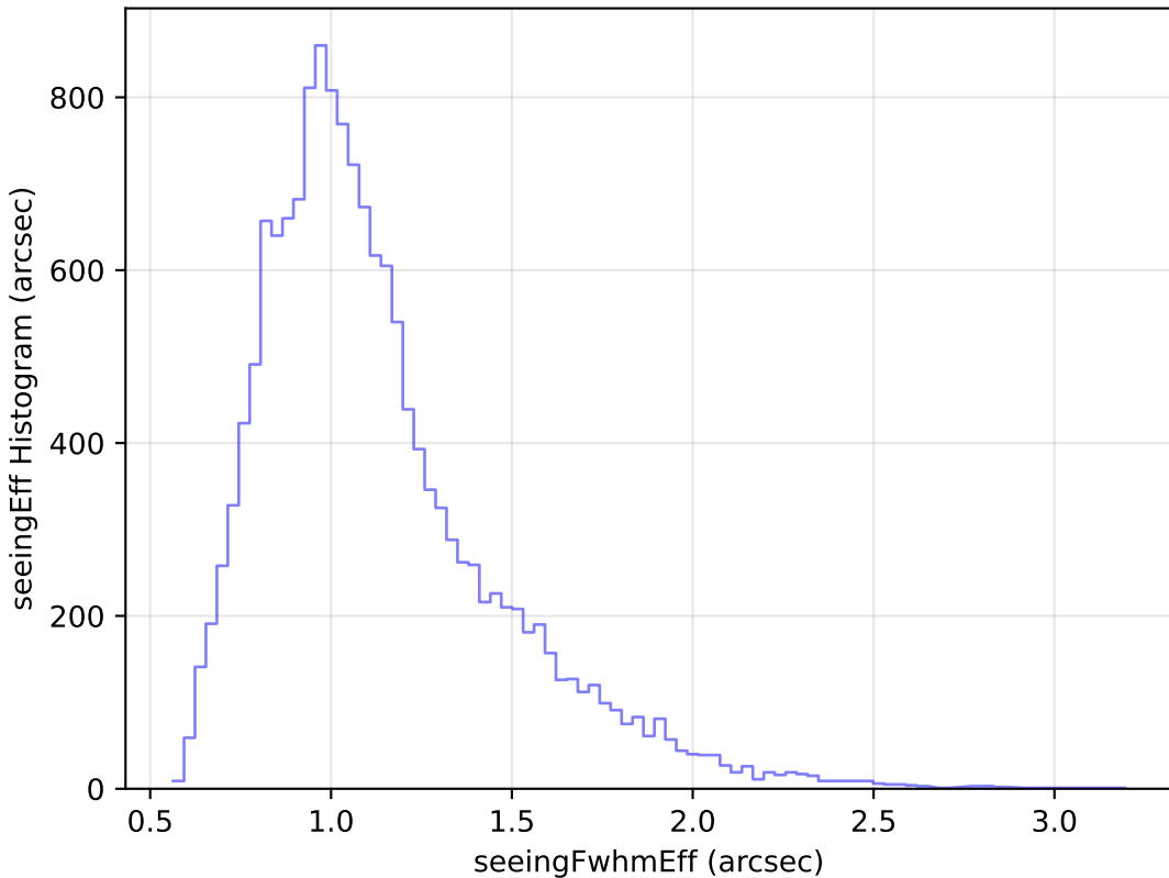
roll_pause_mjdp270_v3.4_10yrs Yr 1 u band: seeingEff Histogram
