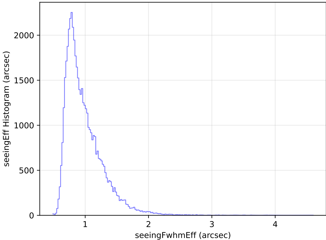
roll_pause_mjdp270_v3.4_10yrs Yr 1 r band: seeingEff Histogram
