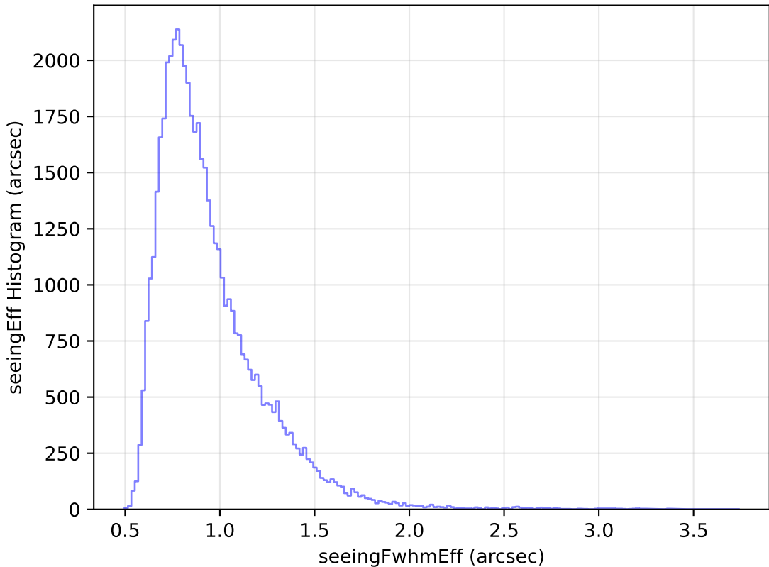
roll_pause_mjdp270_v3.4_10yrs Yr 1 i band: seeingEff Histogram
