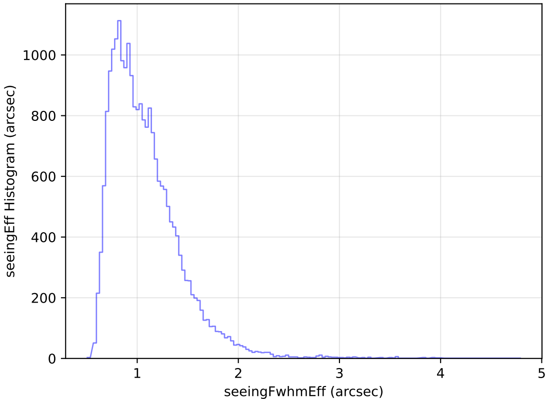
roll_pause_mjdp270_v3.4_10yrs Yr 1 g band: seeingEff Histogram
