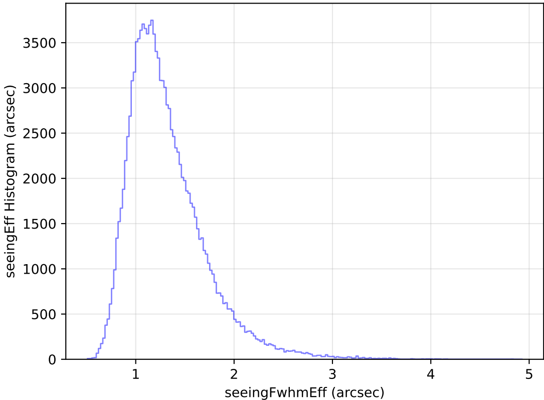
roll_pause_mjdp270_v3.4_10yrs WFD u band: seeingEff Histogram
