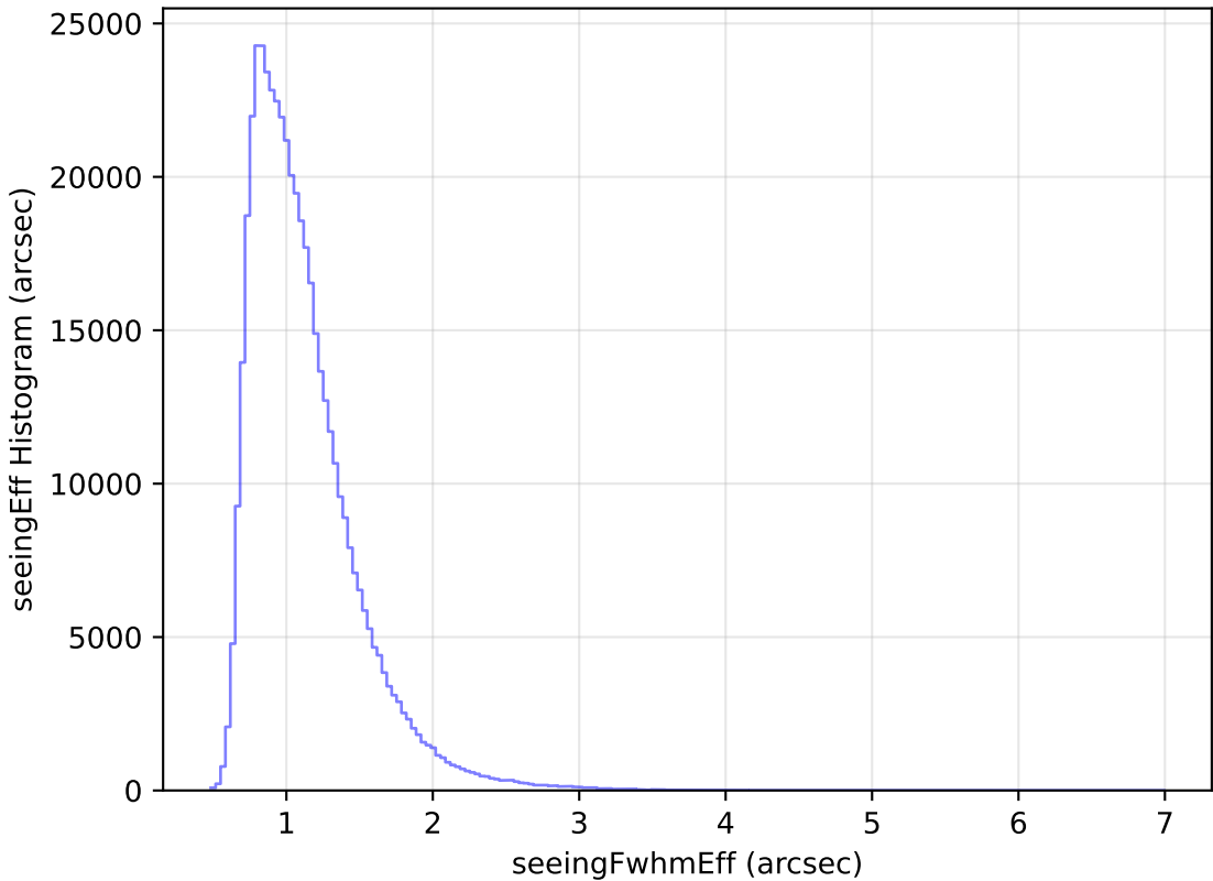
roll_pause_mjdp270_v3.4_10yrs WFD r band: seeingEff Histogram
