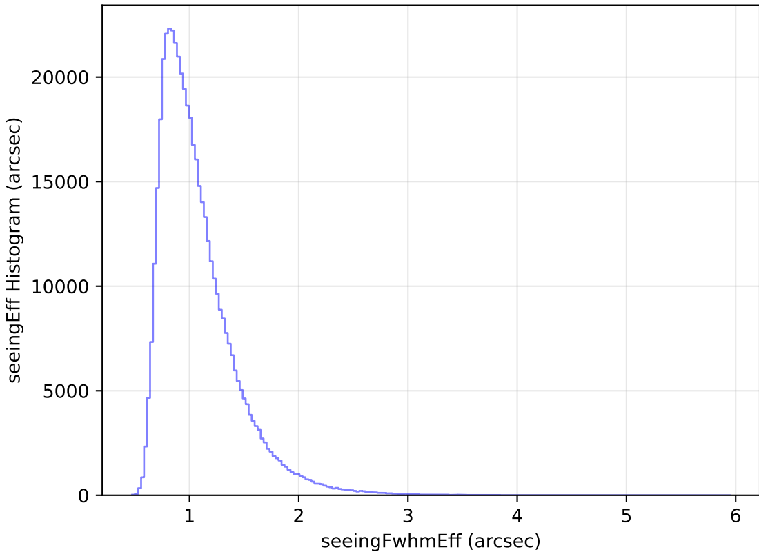
roll_pause_mjdp270_v3.4_10yrs WFD i band: seeingEff Histogram
