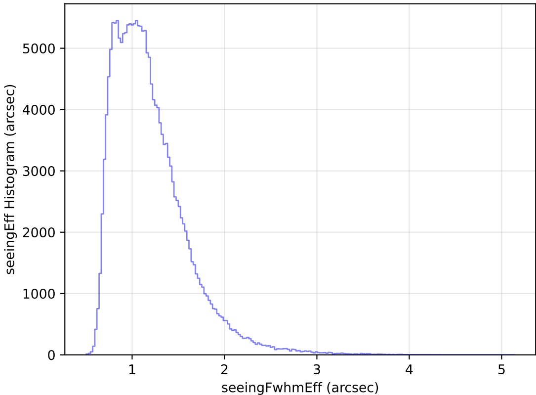
roll_pause_mjdp270_v3.4_10yrs WFD g band: seeingEff Histogram
