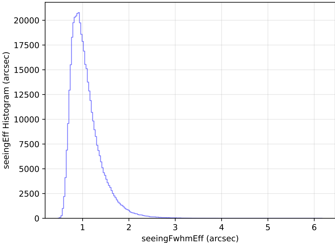
roll_pause_mjdp270_v3.4_10yrs All sky z band: seeingEff Histogram
