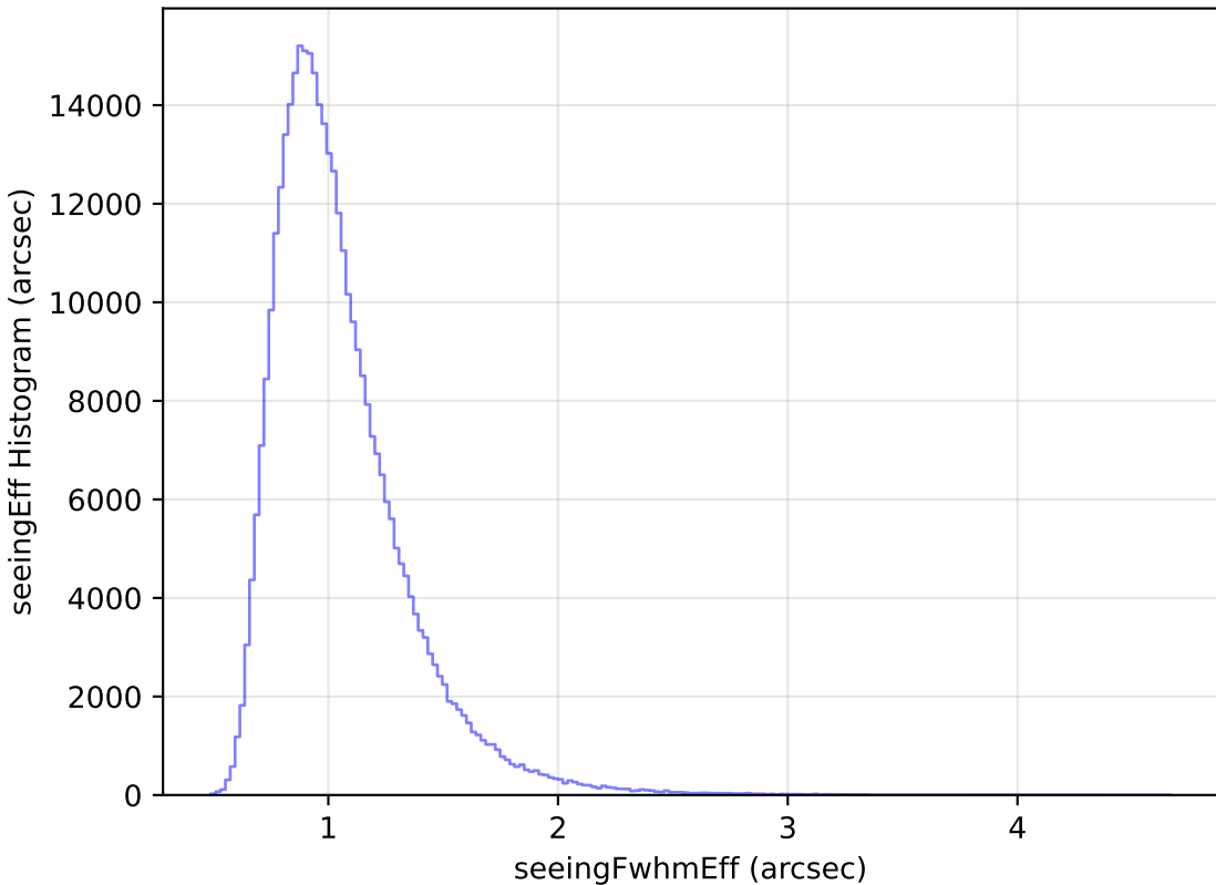
roll_pause_mjdp270_v3.4_10yrs All sky y band: seeingEff Histogram
