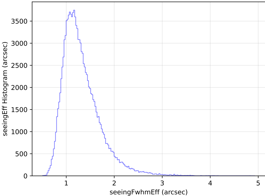
roll_pause_mjdp270_v3.4_10yrs All sky u band: seeingEff Histogram
