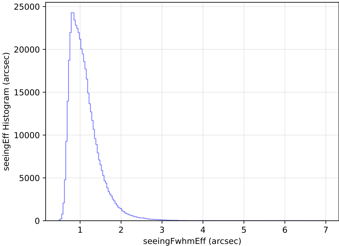
roll_pause_mjdp270_v3.4_10yrs All sky r band: seeingEff Histogram
