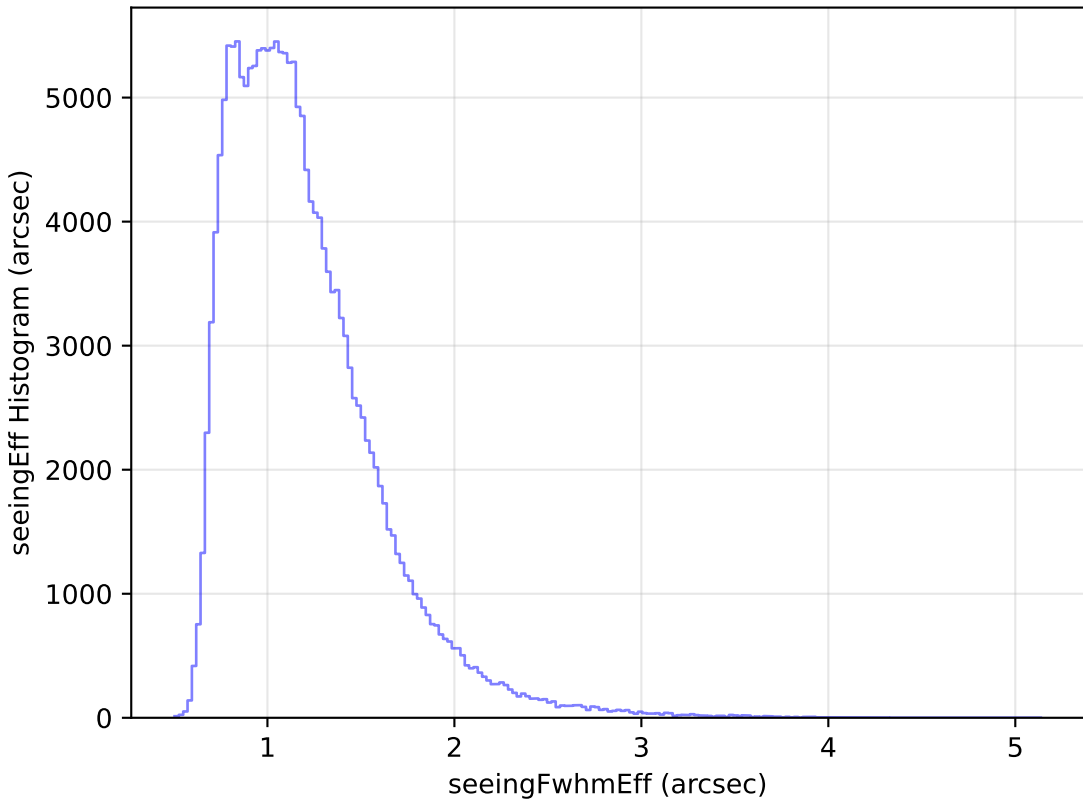
roll_pause_mjdp270_v3.4_10yrs All sky g band: seeingEff Histogram
