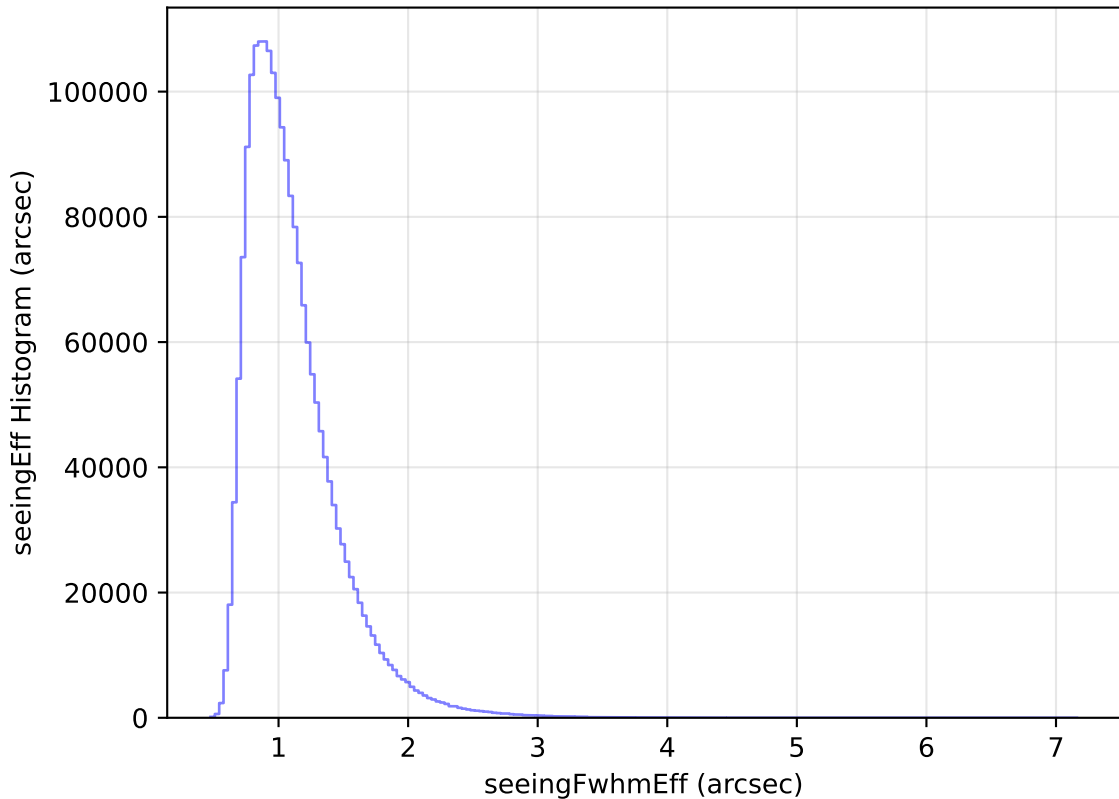
roll_pause_mjdp270_v3.4_10yrs All sky all bands: seeingEff Histogram
