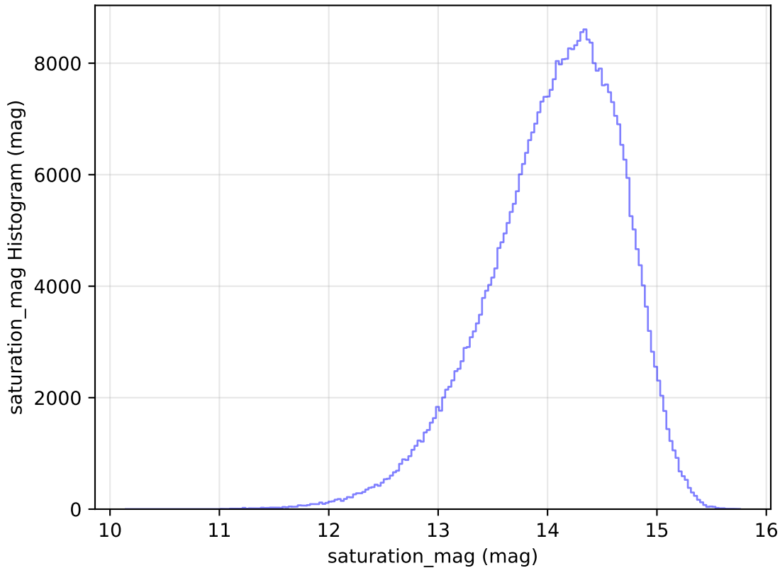
roll_pause_mjdp270_v3.4_10yrs WFD z band: saturation_mag Histogram
