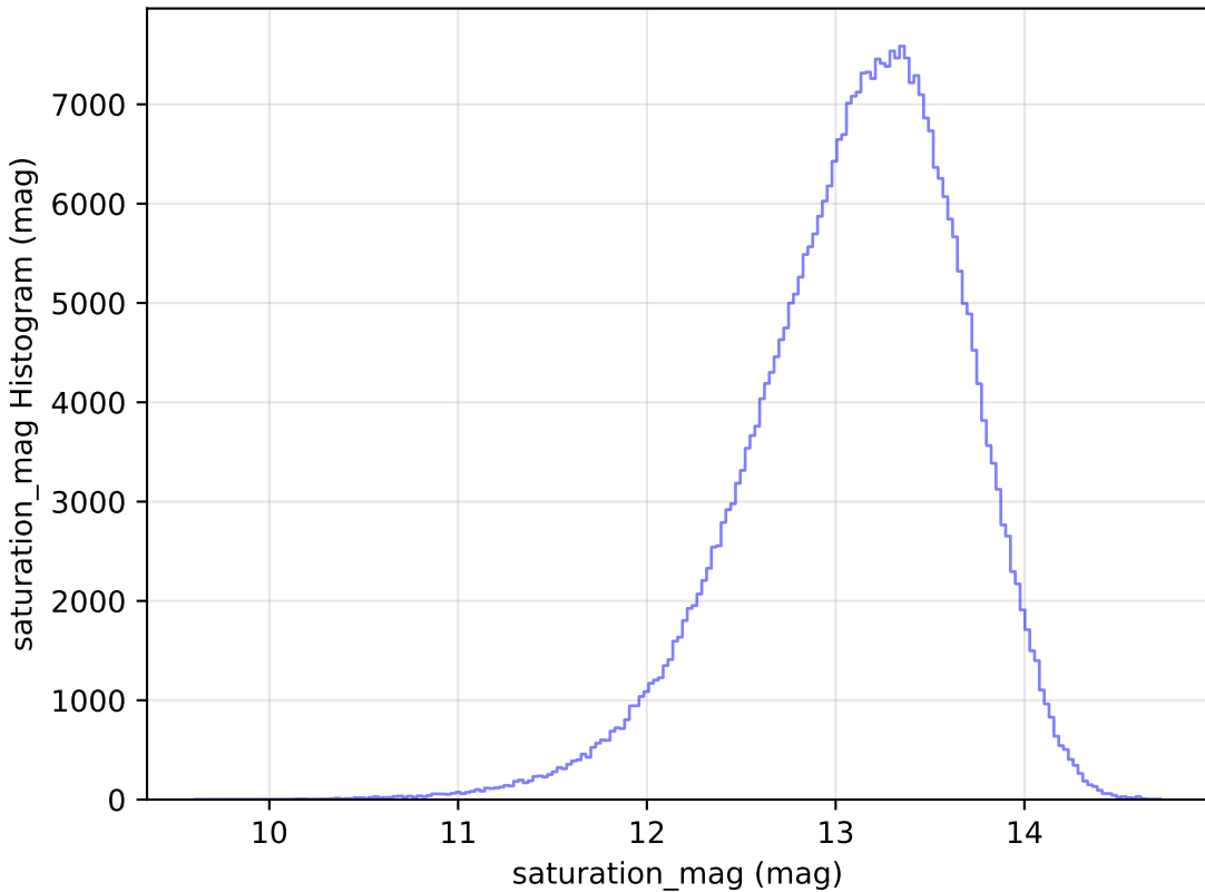
roll_pause_mjdp270_v3.4_10yrs WFD y band: saturation_mag Histogram
