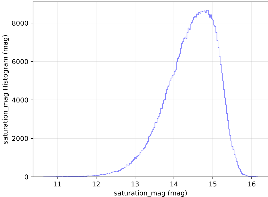
roll_pause_mjdp270_v3.4_10yrs WFD i band: saturation_mag Histogram
