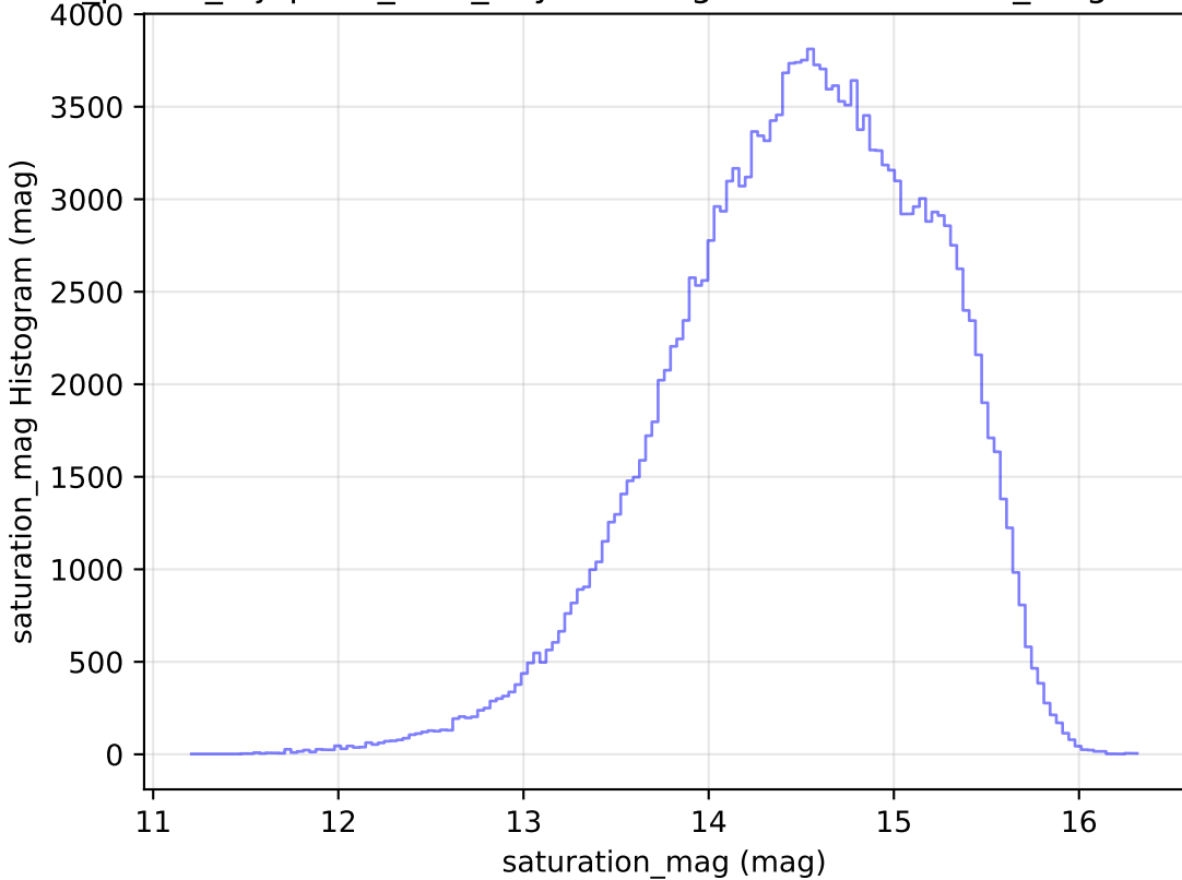
roll_pause_mjdp270_v3.4_10yrs WFD g band: saturation_mag Histogram
