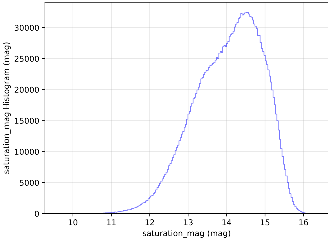
roll_pause_mjdp270_v3.4_10yrs WFD all bands: saturation_mag Histogram
