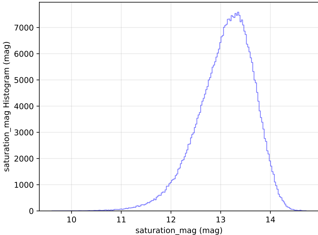
roll_pause_mjdp270_v3.4_10yrs All sky y band: saturation_mag Histogram
