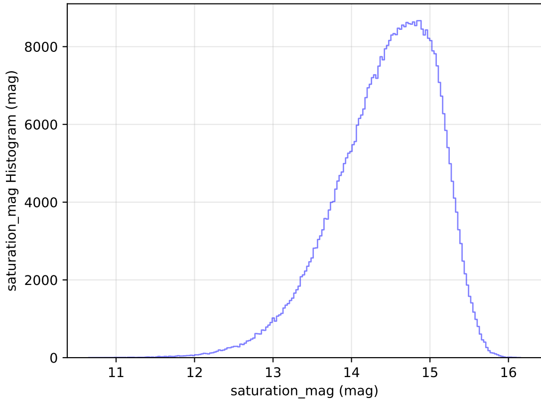
roll_pause_mjdp270_v3.4_10yrs All sky i band: saturation_mag Histogram
