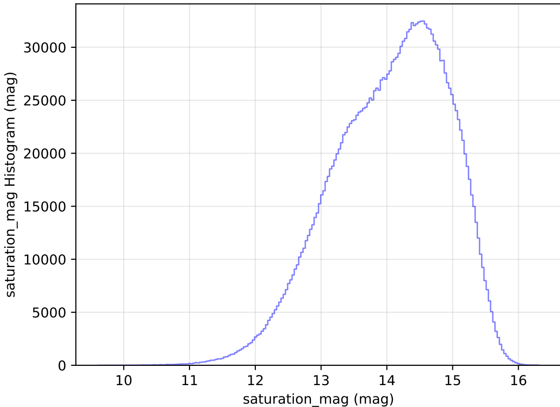
roll_pause_mjdp270_v3.4_10yrs All sky all bands: saturation_mag Histogram
