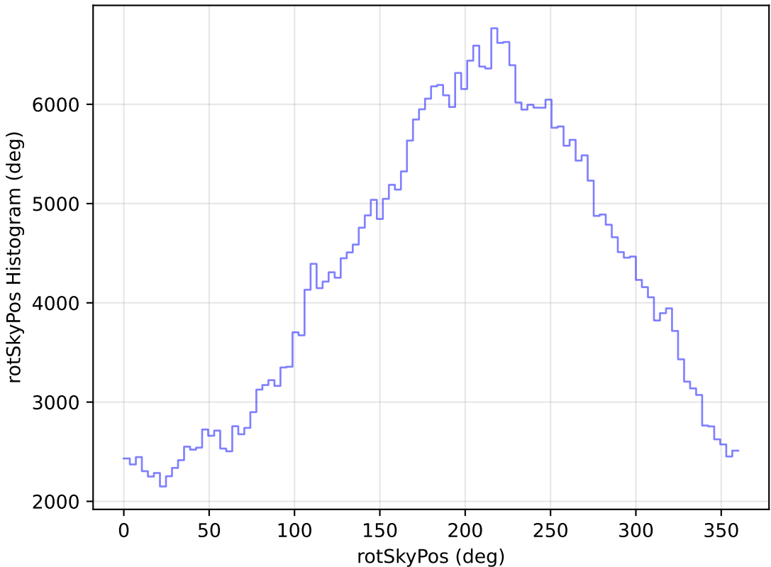
roll_pause_mjdp270_v3.4_10yrs WFD z band: rotSkyPos Histogram
