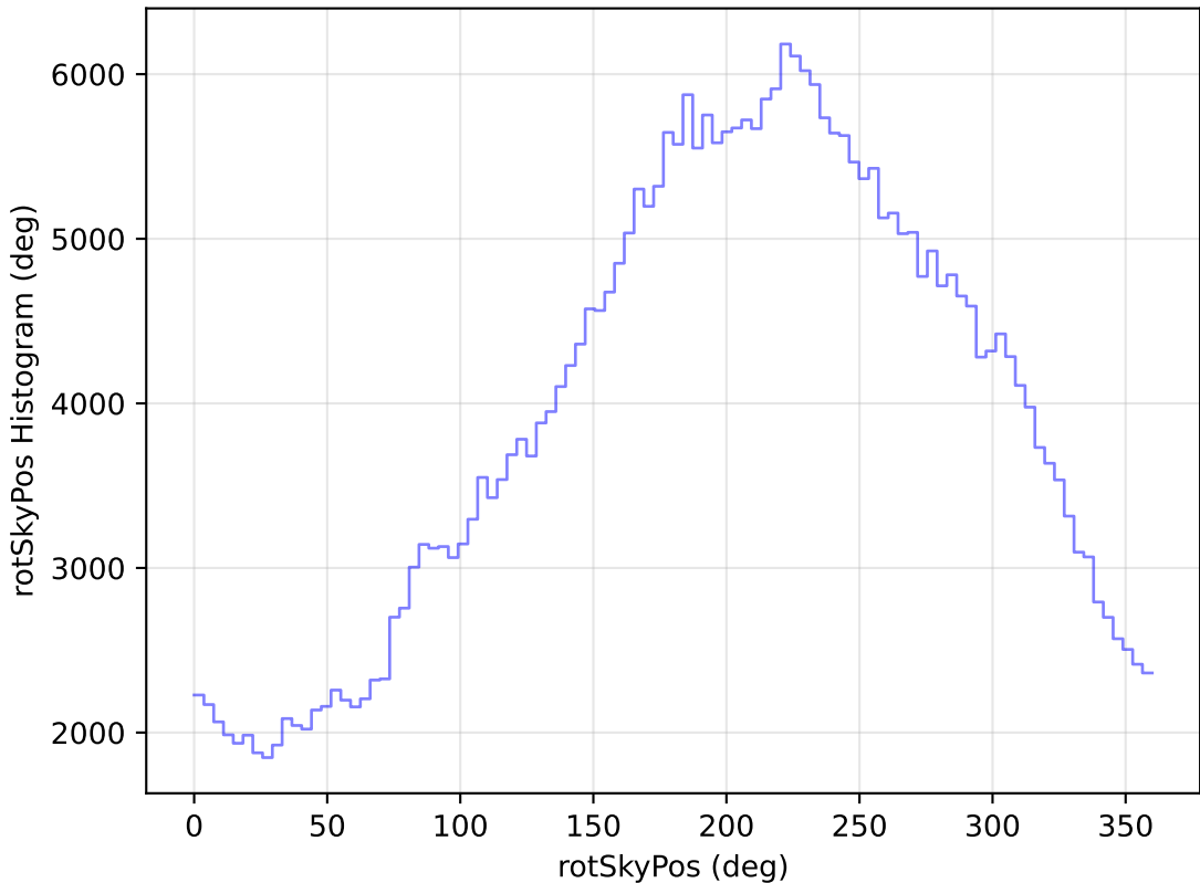
roll_pause_mjdp270_v3.4_10yrs WFD y band: rotSkyPos Histogram
