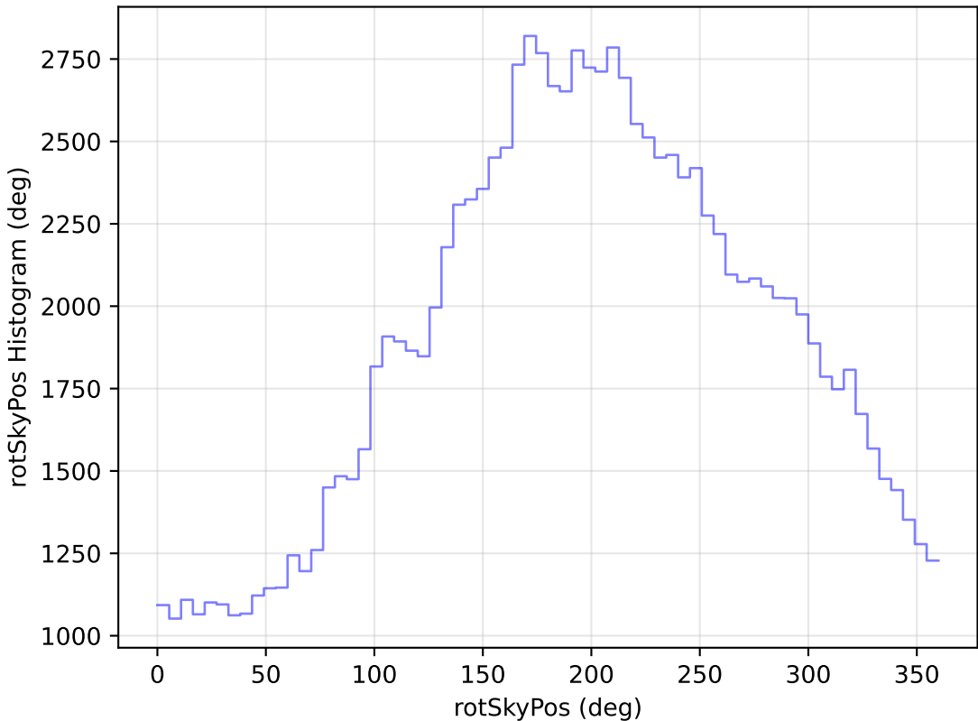
roll_pause_mjdp270_v3.4_10yrs WFD u band: rotSkyPos Histogram
