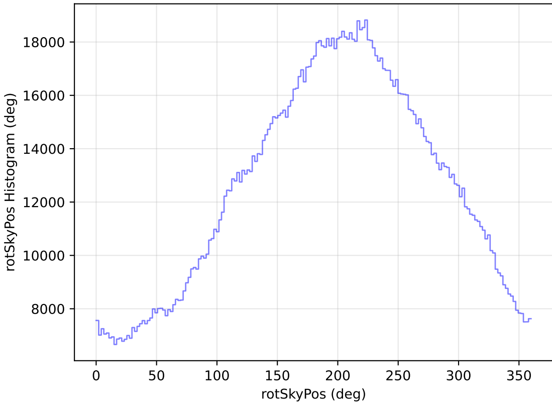
roll_pause_mjdp270_v3.4_10yrs WFD all bands: rotSkyPos Histogram
