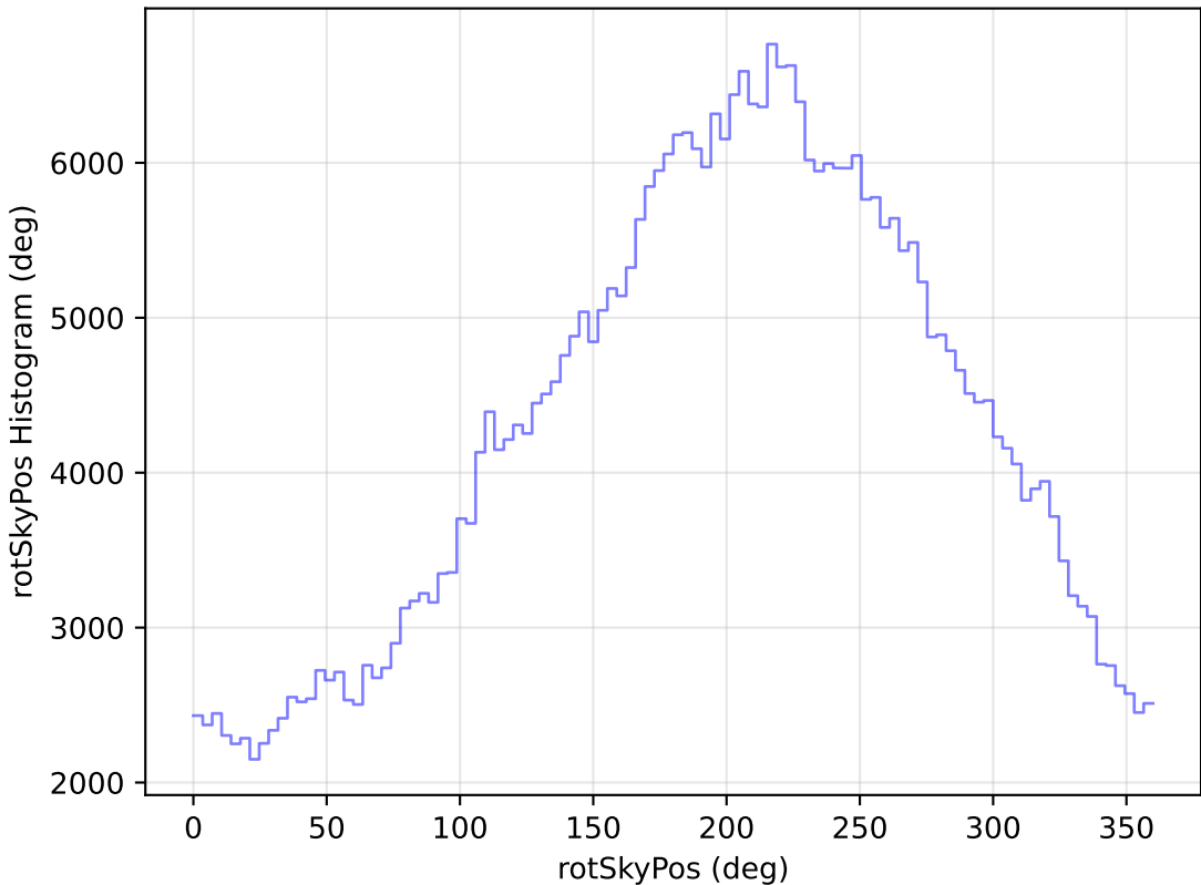
roll_pause_mjdp270_v3.4_10yrs All sky z band: rotSkyPos Histogram
