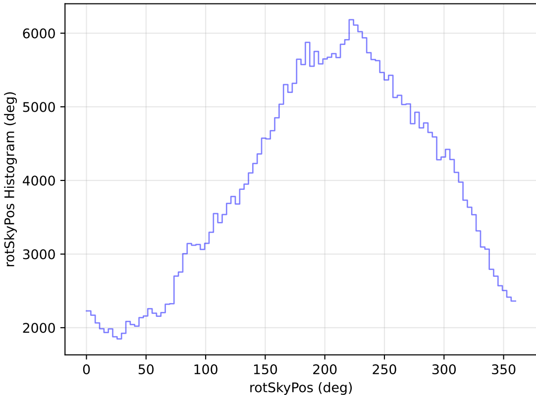
roll_pause_mjdp270_v3.4_10yrs All sky y band: rotSkyPos Histogram
