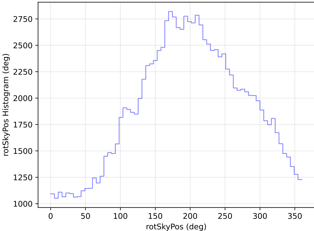
roll_pause_mjdp270_v3.4_10yrs All sky u band: rotSkyPos Histogram
