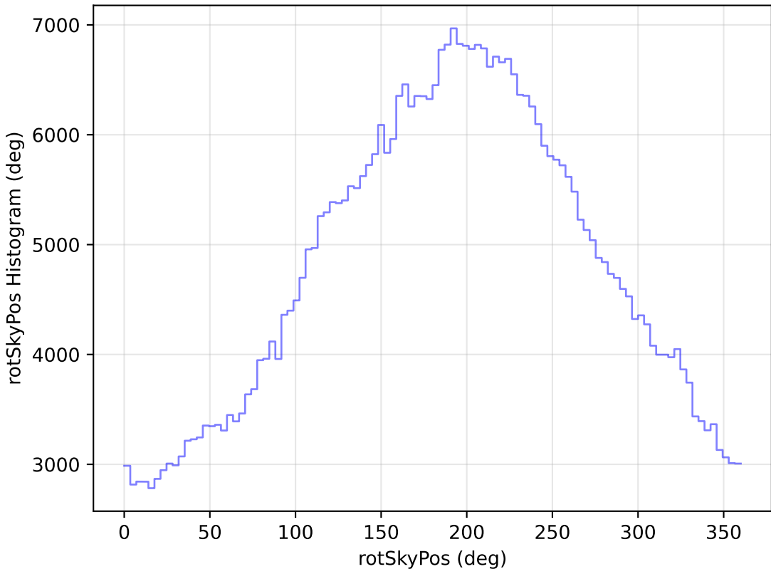
roll_pause_mjdp270_v3.4_10yrs All sky r band: rotSkyPos Histogram
