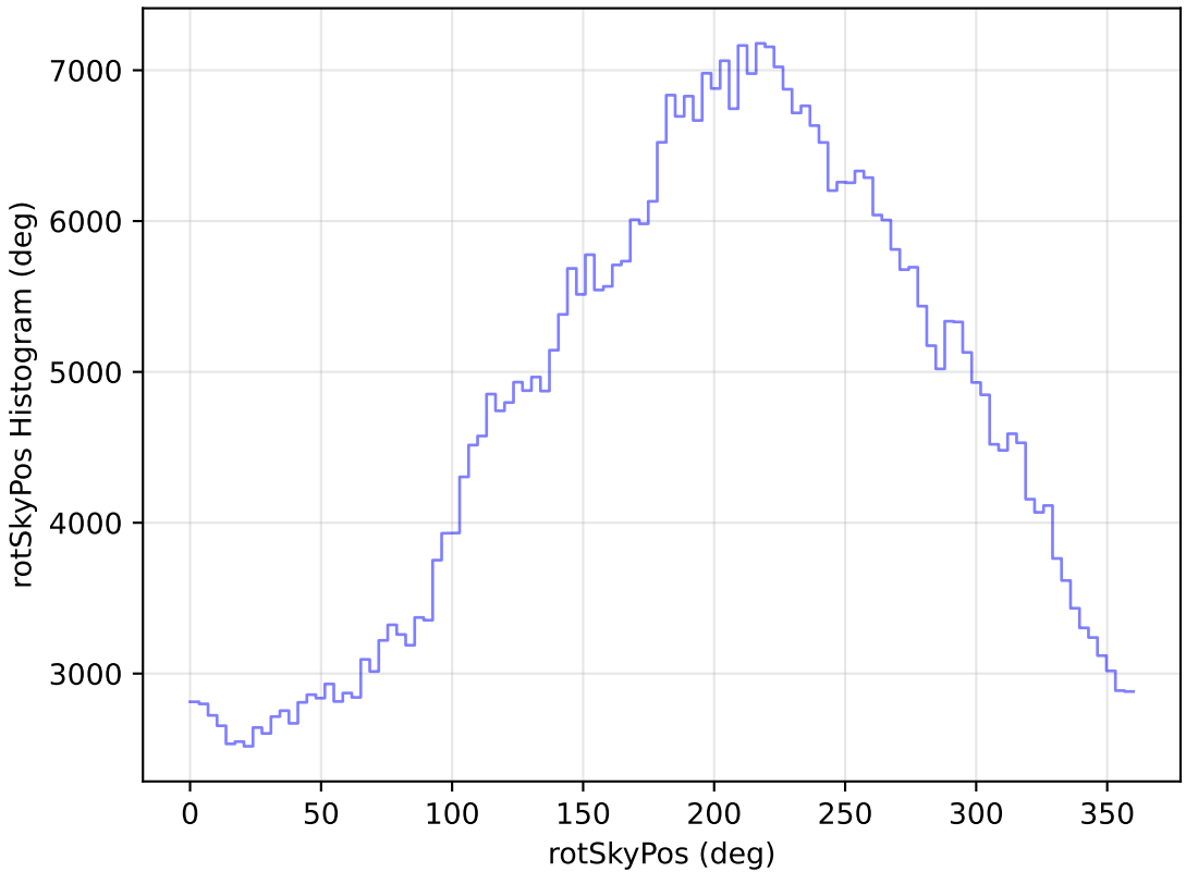
roll_pause_mjdp270_v3.4_10yrs All sky i band: rotSkyPos Histogram
