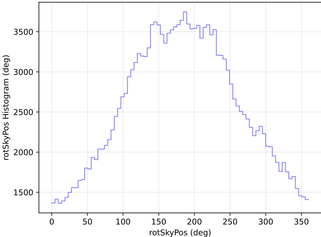
roll_pause_mjdp270_v3.4_10yrs All sky g band: rotSkyPos Histogram
