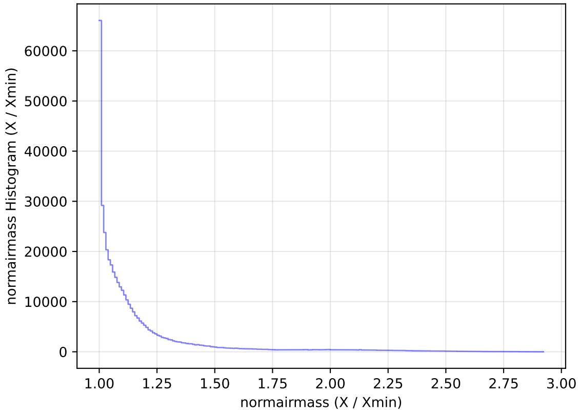
roll_pause_mjdp270_v3.4_10yrs WFD z band: normairmass Histogram
