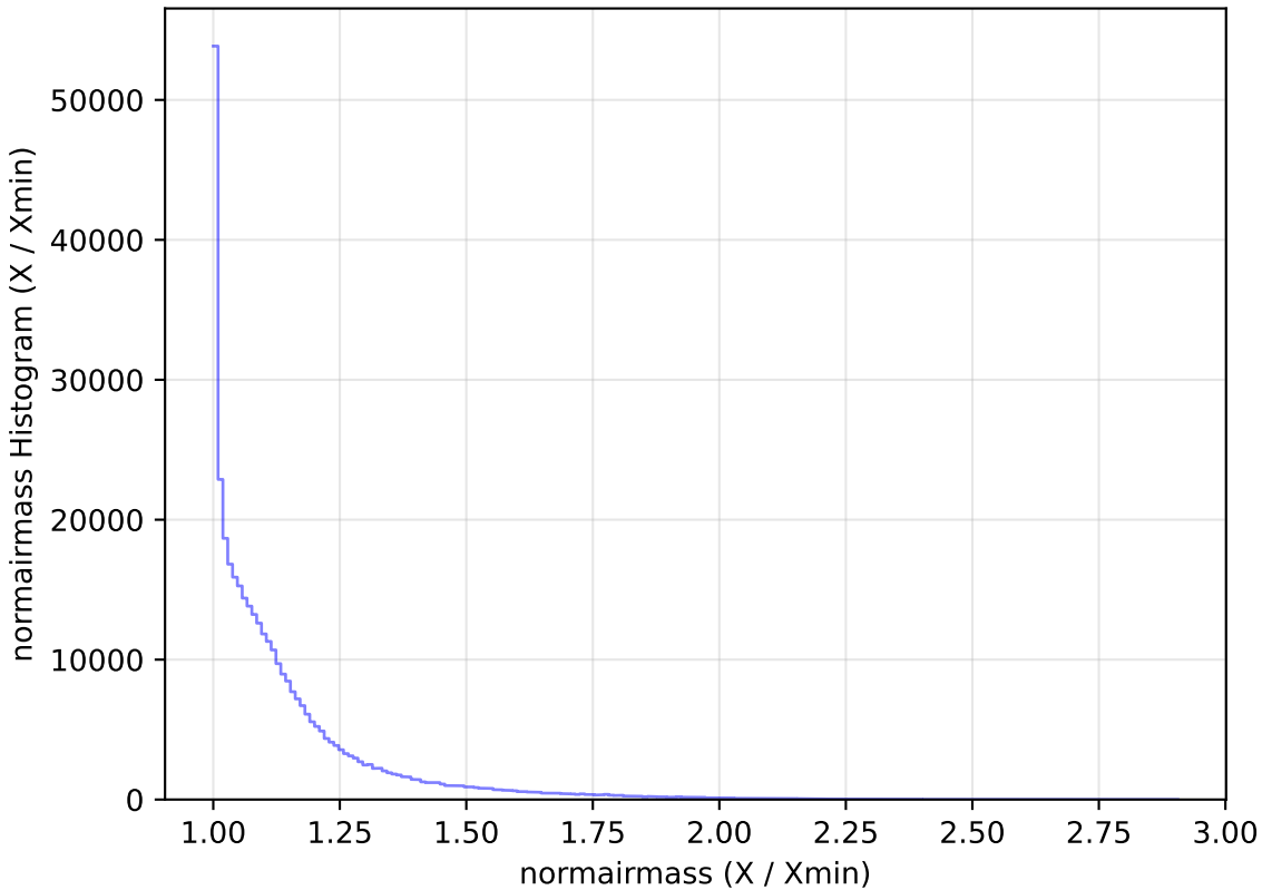
roll_pause_mjdp270_v3.4_10yrs WFD y band: normairmass Histogram
