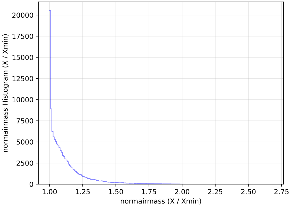
roll_pause_mjdp270_v3.4_10yrs WFD u band: normairmass Histogram
