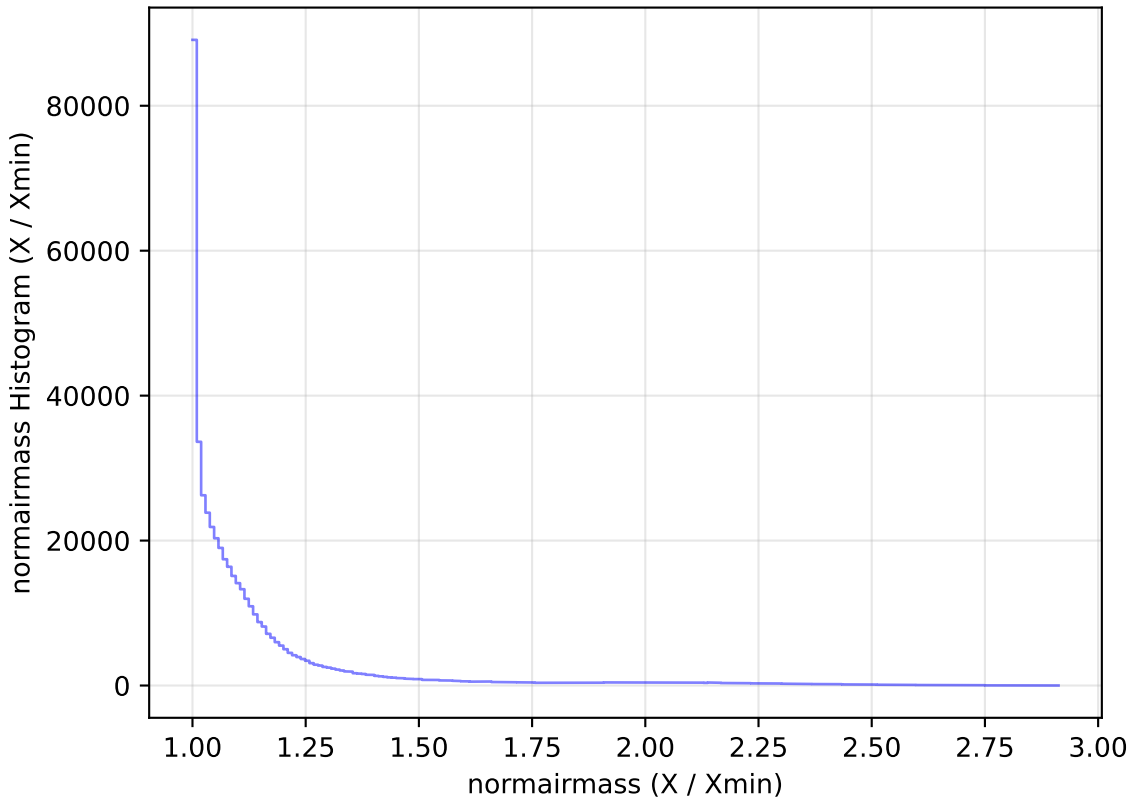
roll_pause_mjdp270_v3.4_10yrs WFD i band: normairmass Histogram
