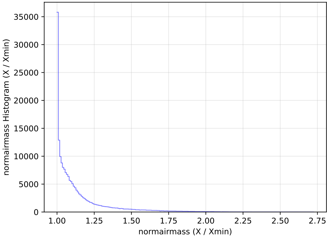
roll_pause_mjdp270_v3.4_10yrs WFD g band: normairmass Histogram
