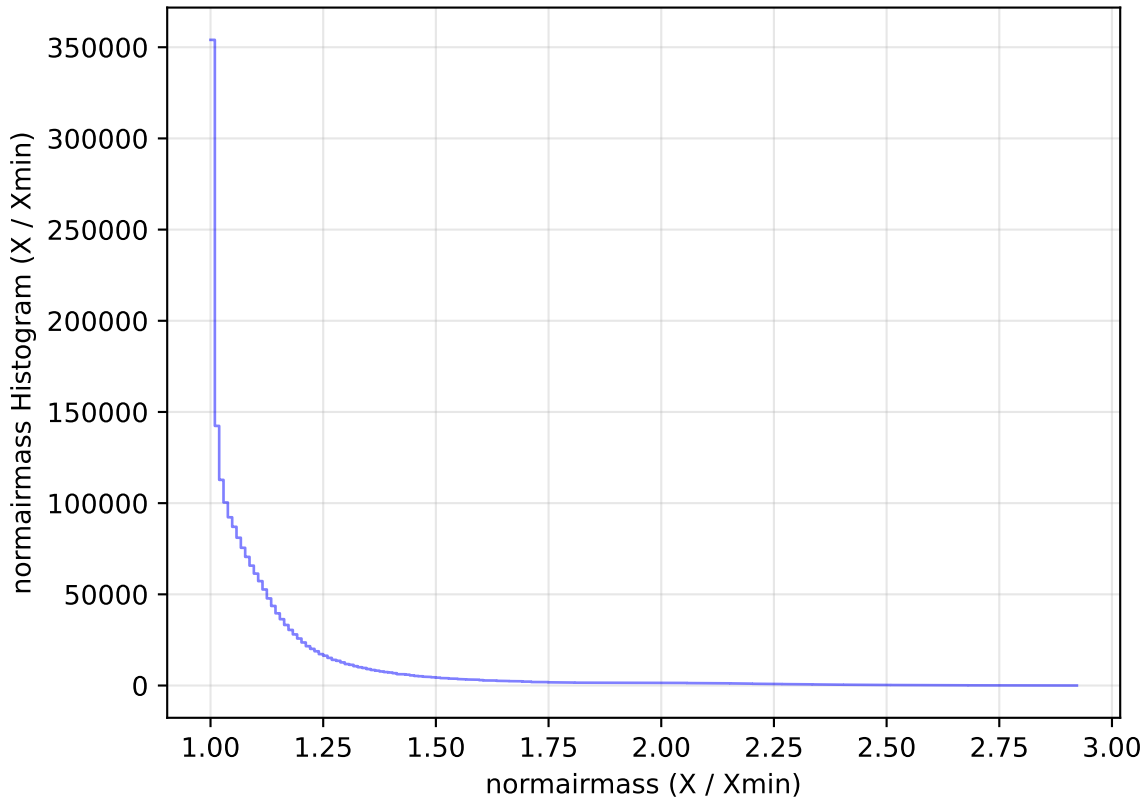
roll_pause_mjdp270_v3.4_10yrs WFD all bands: normairmass Histogram
