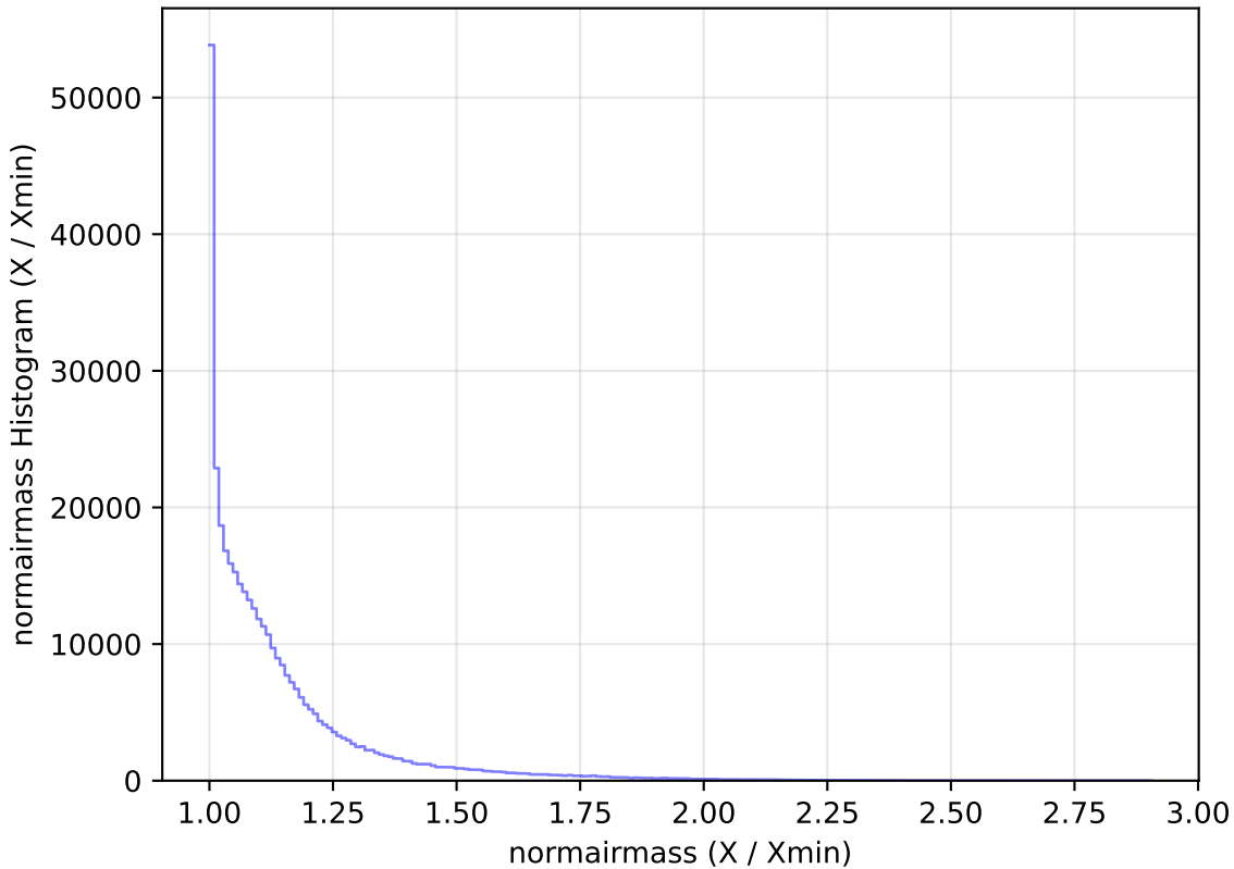
roll_pause_mjdp270_v3.4_10yrs All sky y band: normairmass Histogram
