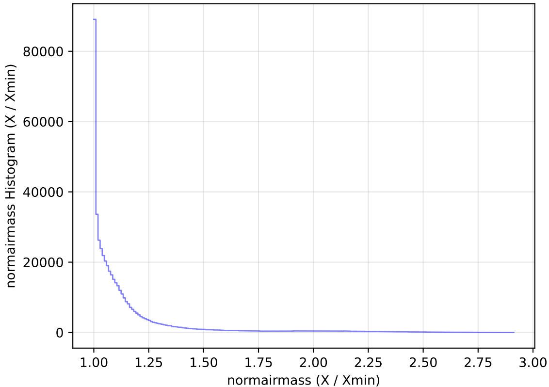
roll_pause_mjdp270_v3.4_10yrs All sky i band: normairmass Histogram
