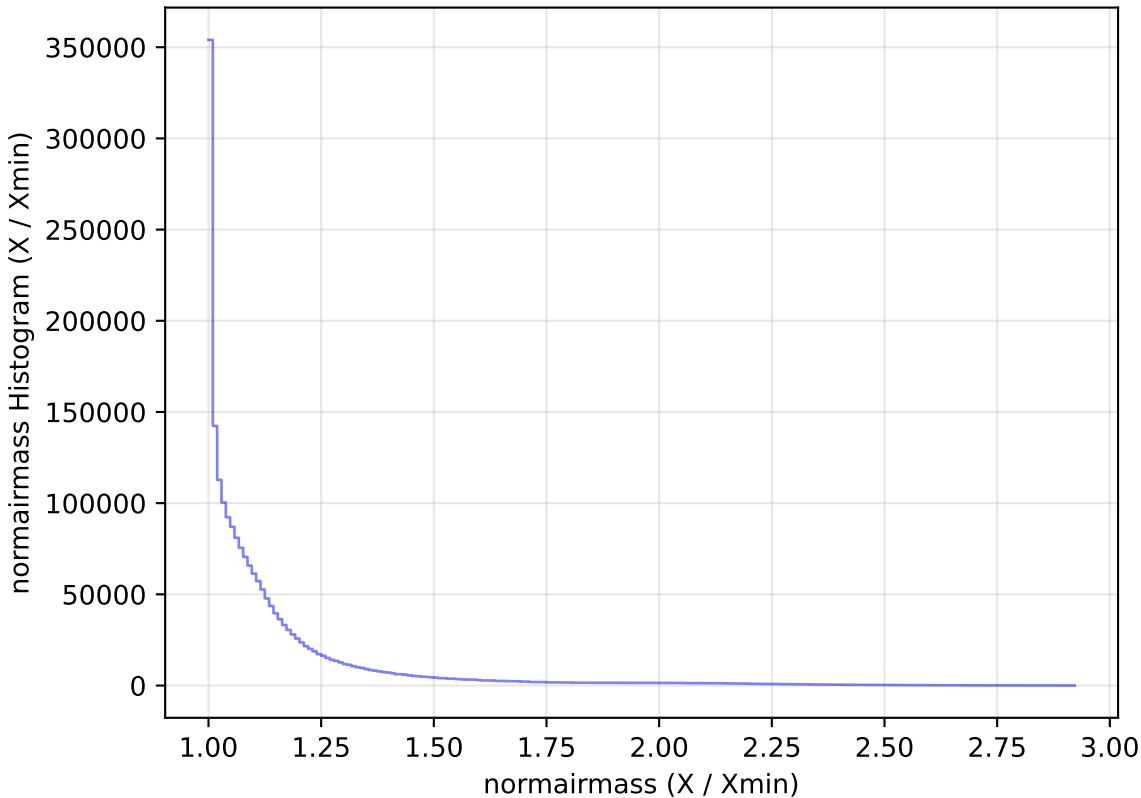
roll_pause_mjdp270_v3.4_10yrs All sky all bands: normairmass Histogram
