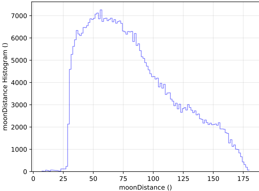
roll_pause_mjdp270_v3.4_10yrs WFD z band: moonDistance Histogram
